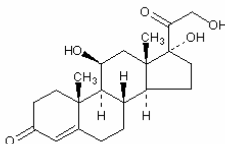
Fig.7 Hydrocortisone
