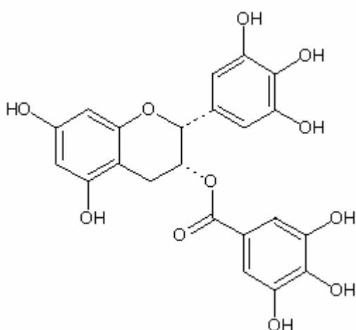
Fig. 19 Epigallocatechin-3-O-gallate
