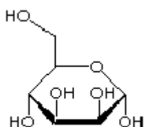
α-D-Mannose
