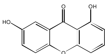
Fig 41. Calaphyllin-B
