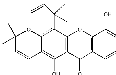
Fig 36. Caloxanthone C
