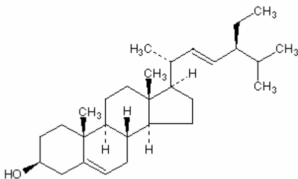
Fig.5 Stigmasterol
