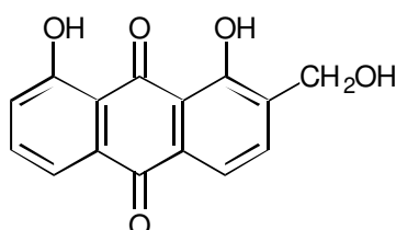
Fig. 49 Aloetic acid
