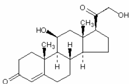
Fig.5 Stigmasterol
