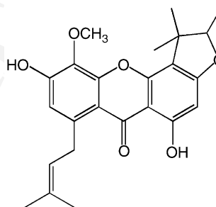
Caloxantone A
