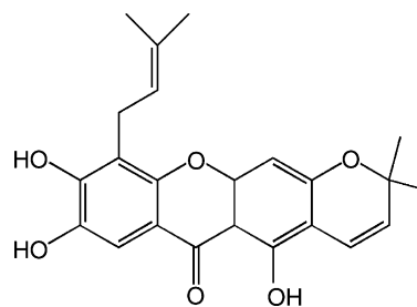
Caloxanthone B
